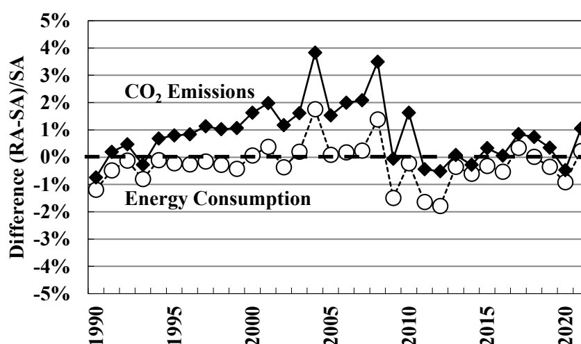
Figure 3-1 Trends in difference of energy consumption and CO 2 emissions
